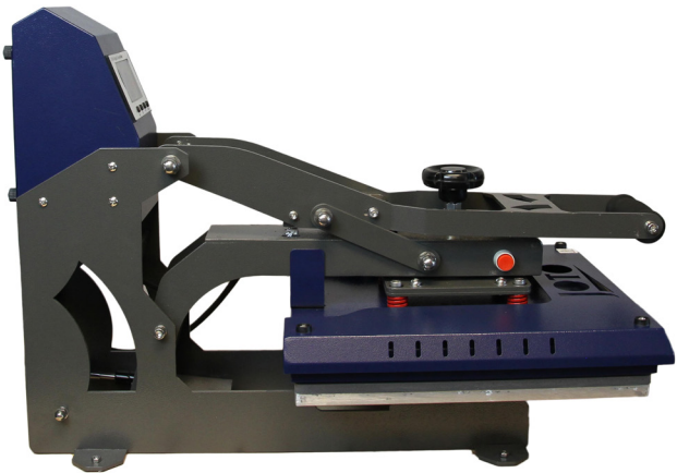
LEFT VIEW
