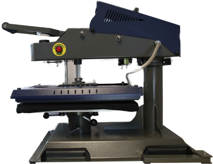
RIGHT VIEW
